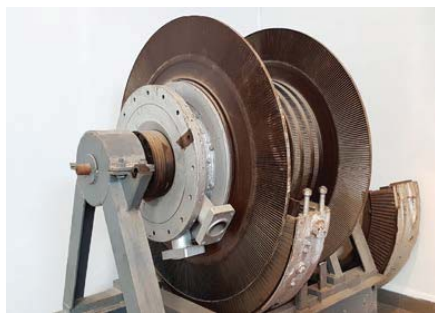
Figure 6 - Ljungström steam turbine, 1928
