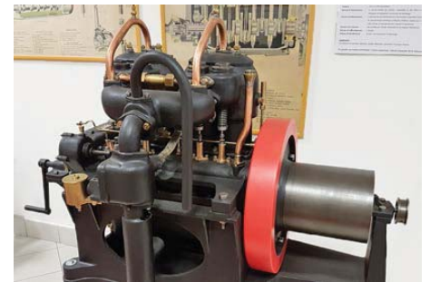
Figure 9 - Oreglia &amp; Co., four-cylinder petrol engine, ca. 1910-1920
